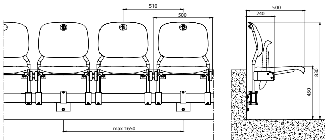
BREGENZ Type B – supporting construction fitted to the riser with the use of a bracket and a bar
