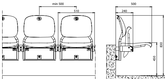
BREGENZ Type A – supporting construction fitted individually to the riser
