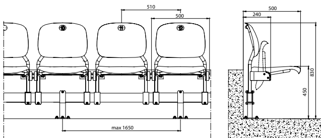
BREGENZ Type C – supporting construction fitted to the riser with the use of legs and a bar
